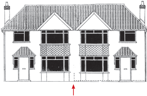
Figure 6: Vertical DPC Between Two Houses
