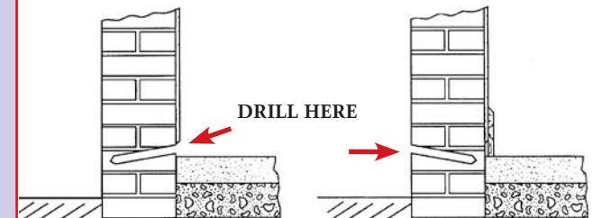
Figure 1: Internal Drilling
