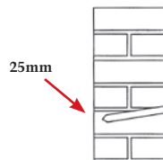
Figure 8: Drilling to within 25mm of Wall Thickness
