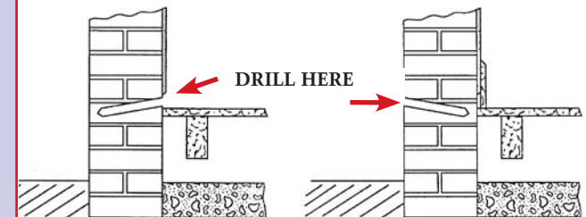
Figure 3: Internal Drilling
