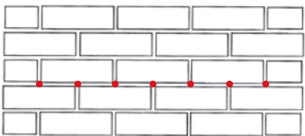
Figure 7: Drilling 113mm Centres
